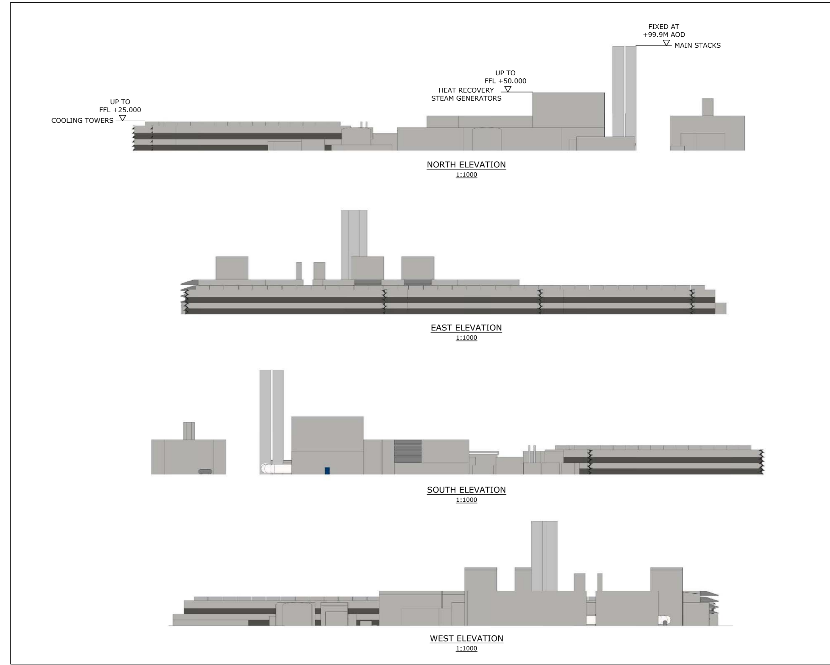
SHEET 6 of 6 - ELEVATIONS MULTI SHAFT
