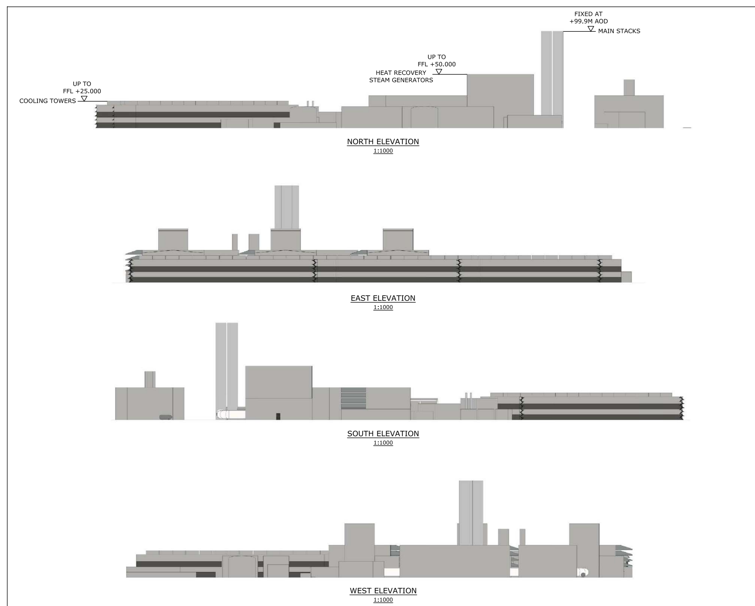
SHEET 3 of 6 - ELEVATIONS SINGLE SHAFT
