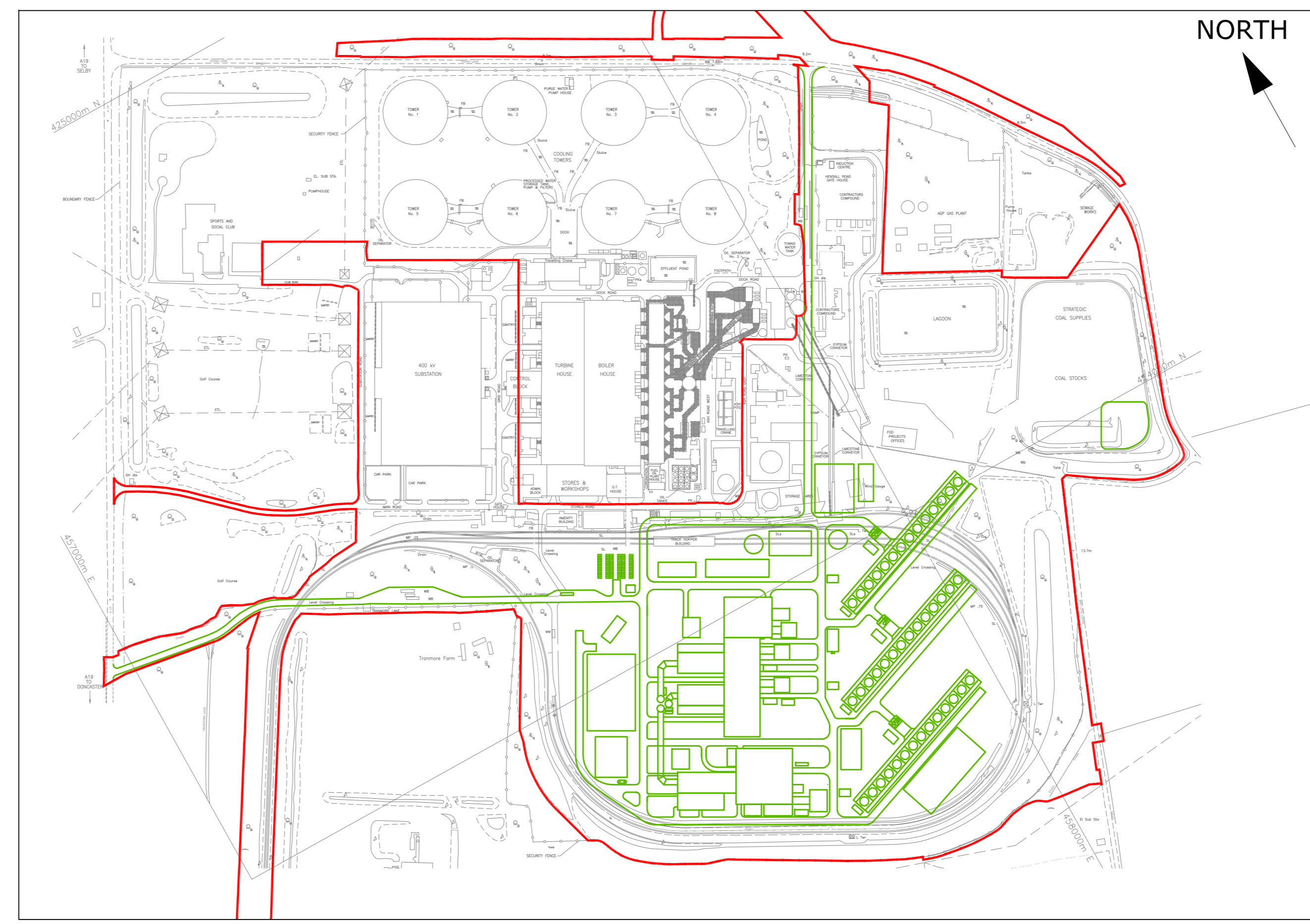
SHEET 4 of 6 - PLAN VIEW MULTI SHAFT
